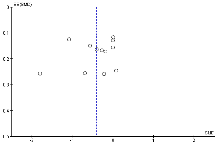
Funnel plot of Overall Studies
